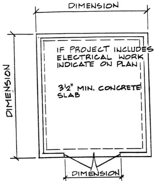
FOUNDATION & FLOOR PLAN SCALE: 1/4" = 1'-0"
