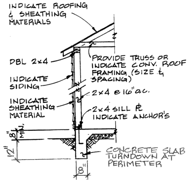
TYPICAL WALL SECTION SCALE: 3/4" = 1'-0"
